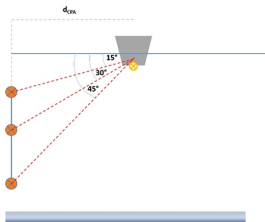
Fig. 5.3.2 (a) Recommended array deployment for deep water (Ref. ISO 17208-1)
