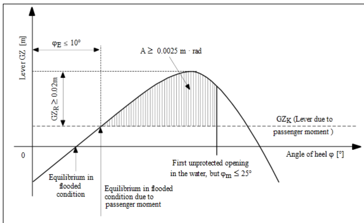
Figure 4.5: Damage Stability
