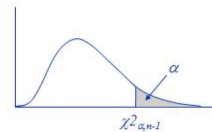
Figure 2.2. Chi-square distribution
