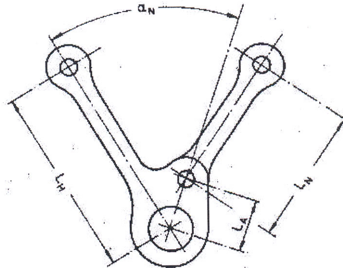
Fig. 2 : Articulated-type connecting-rod
