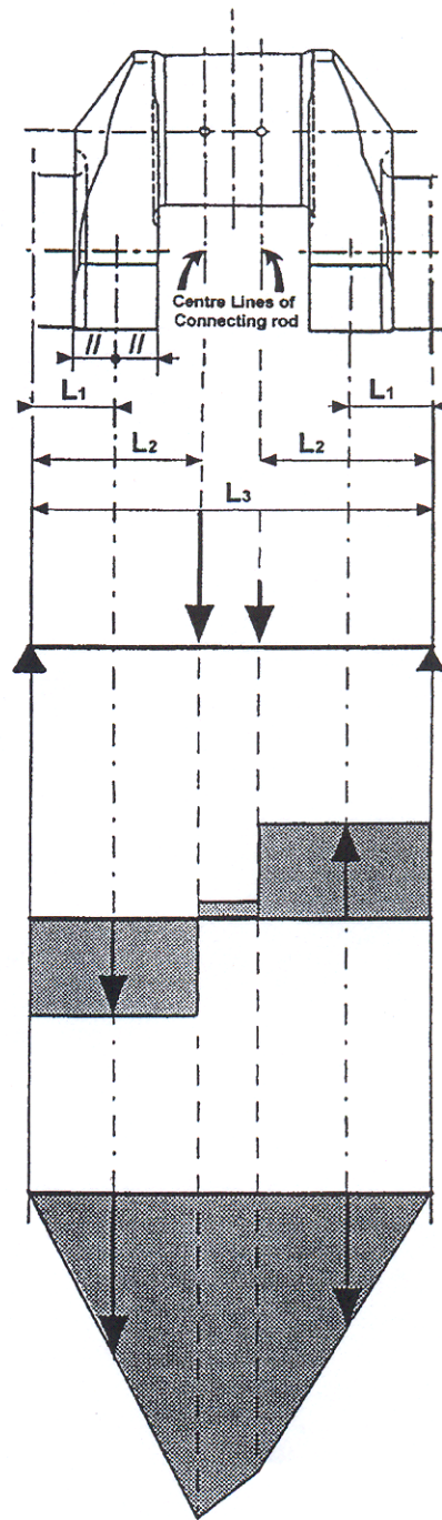
Fig.4 : Crankthrow for Vee-engine with 2 adjacent Connecting-rods
