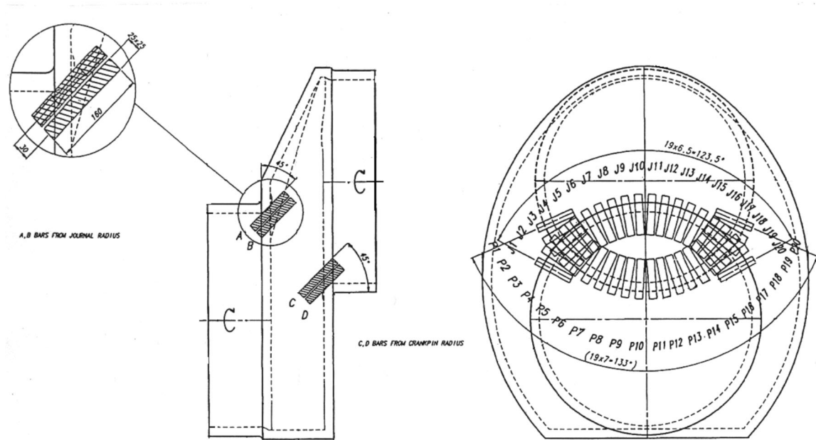
Figure 3.1. Specimen locations in a crank throw
