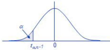
Figure 2.1. Student's t-distribution
