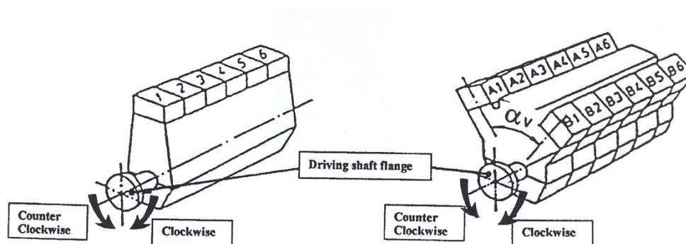
Fig.1 : Designation of the cylinders
